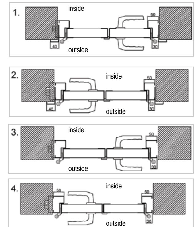
Side Hinged Garage Door fitting and opening option
